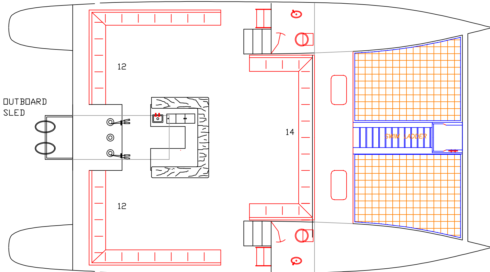
STUDY DRAWING; GCY 44, OUTBOARDS ON SLED, 38 SEATS, 60 PASSENGER CAPACITY
